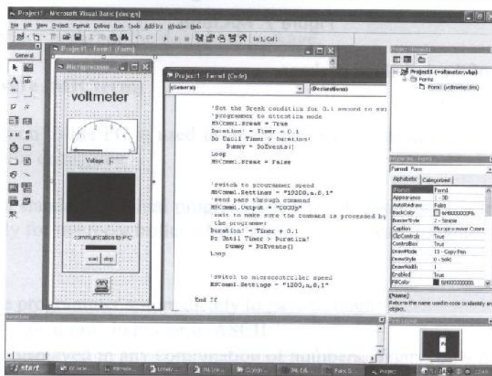
Figure 8. Visual Basic.
