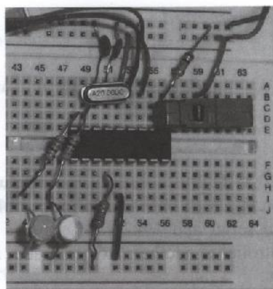
Figure 197. Demo project for the 16F628.
