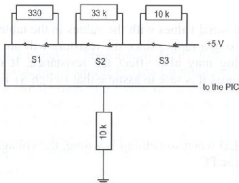
Figure 49. Voltage divider.
