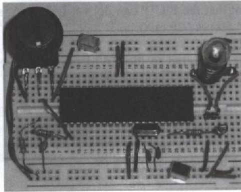
Figure 175. Connecting a 50 mA light bulb to a PIC™.
