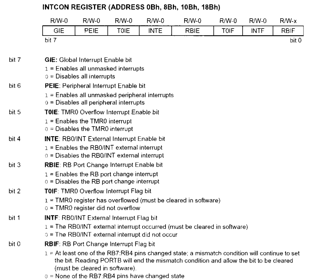
Figure 150. INTCON register.
