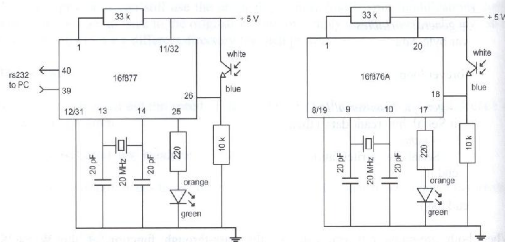
Figure 211. Infrared serial set up.
