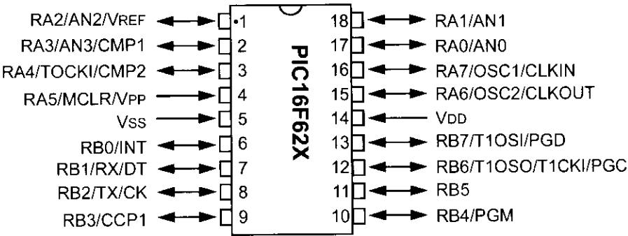
Figure 194. Pin layout of the 16F628.
