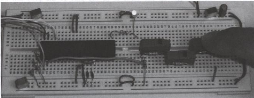
Figure 52. Silent alarm in action.
