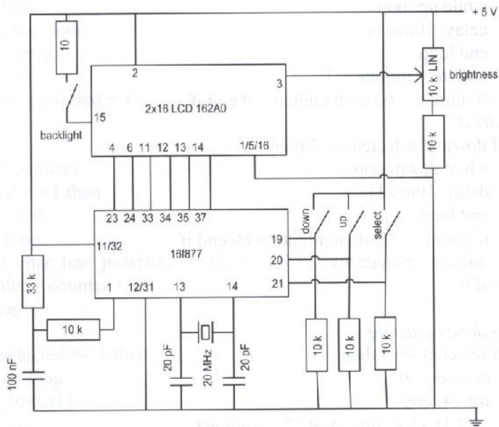
Figure 158. Digital clock.
