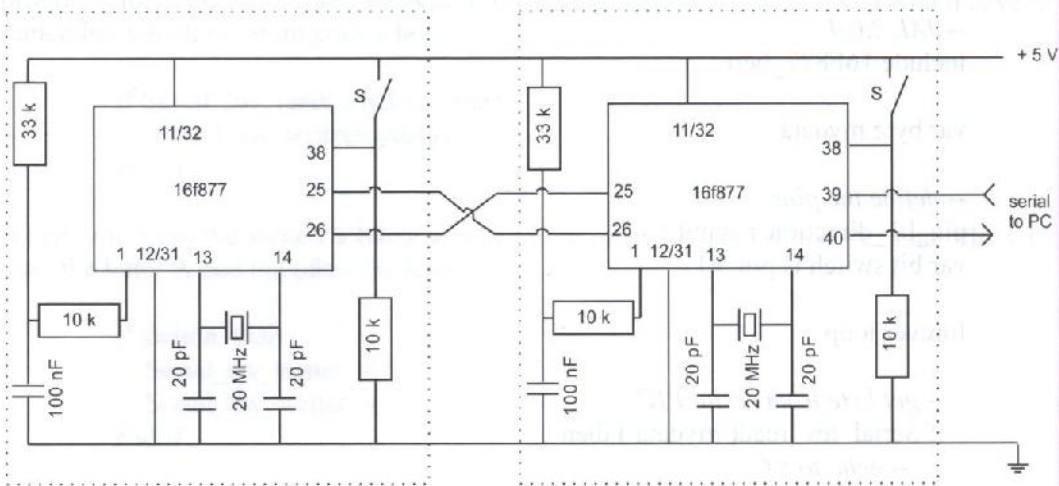
Figure 133. Hardware and software serial connection.
