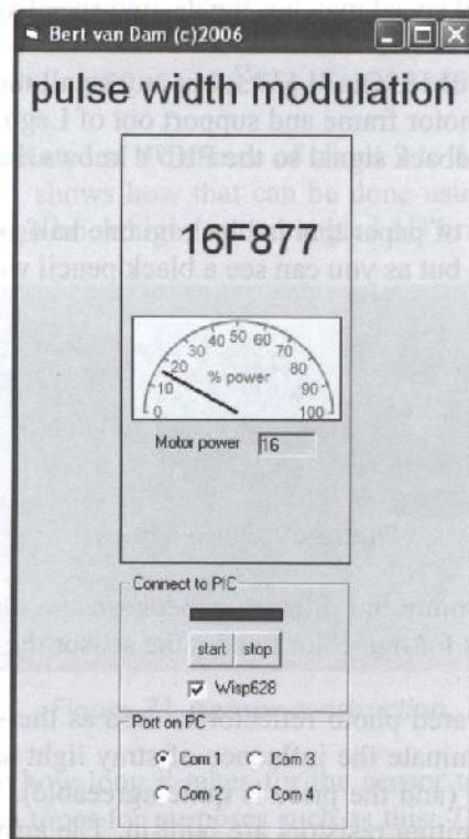
Figure 68. VB program
