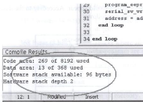
Figure 119. Compiler result.
