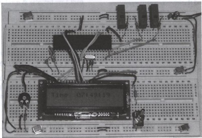
Figure 159. The digital clock is operational.
