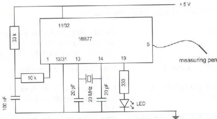
Figure 40. Voltmeter.
